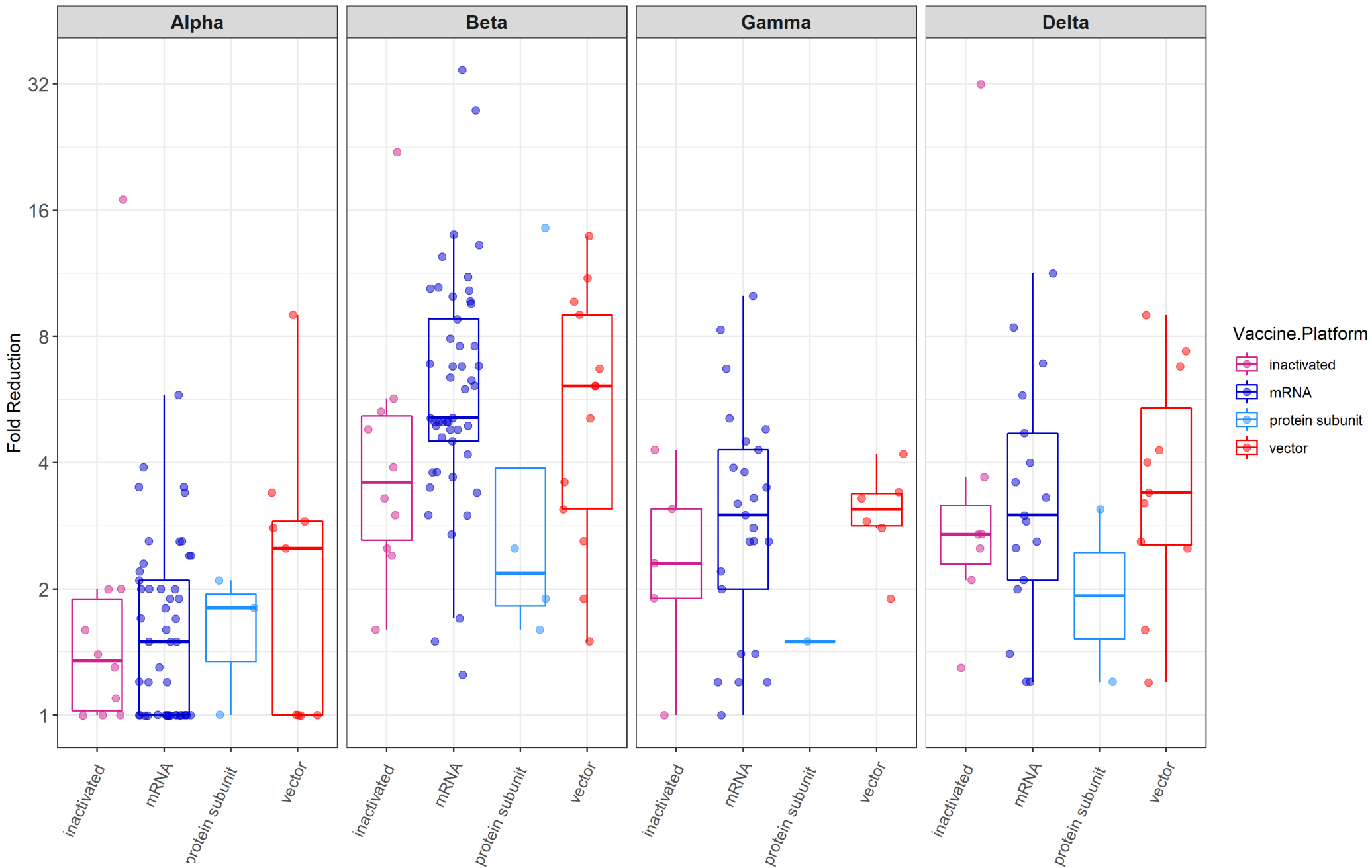
Fold Reduction in NAbs by SARS-CoV-2 Variant of Concern and Vaccine Platform, Box Plot
